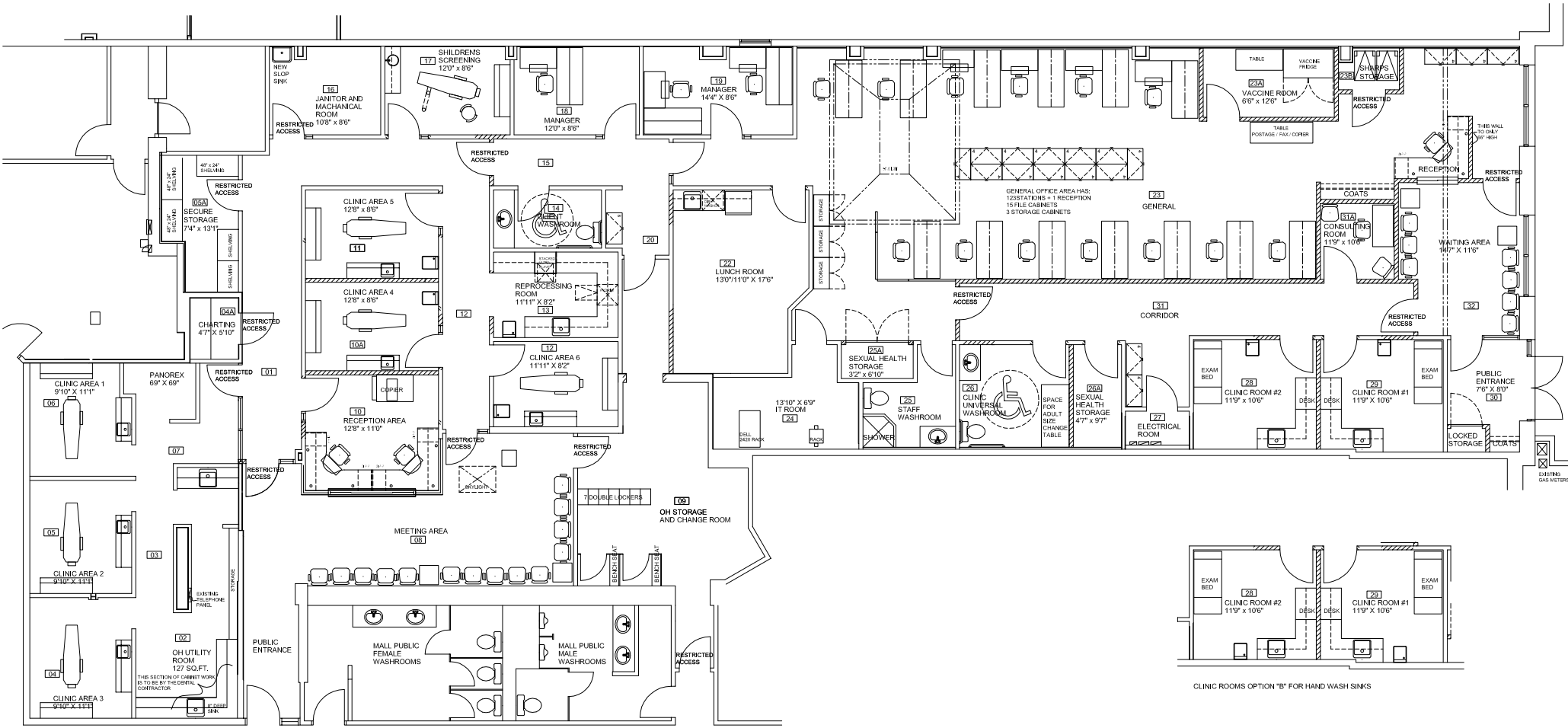
REVISED LAYOUT PLAN; 80 BRADFORD 18-03-22 revision #7
