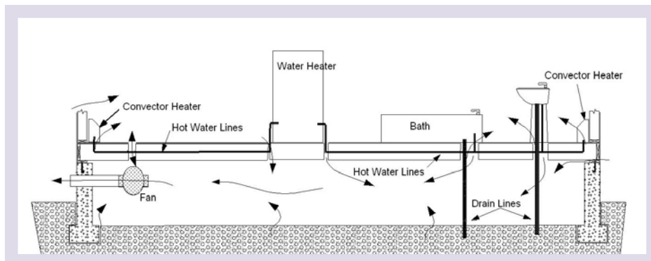
Figure 14 – Crawlspace Exhaust
