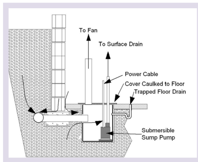
Figure 12 – Sump Exhaust
